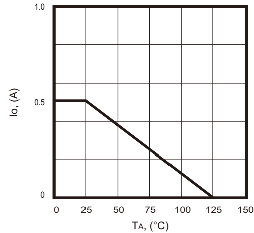
Fig.4 - Derating Curve
